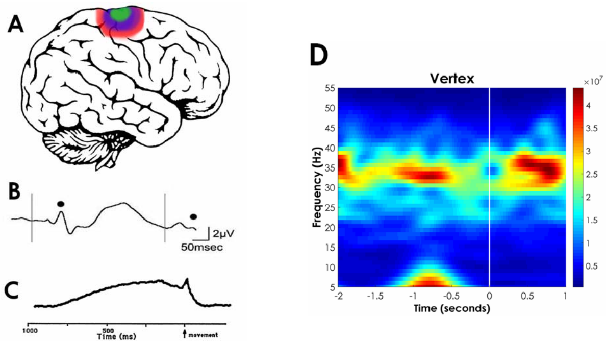
Figure 1. Sensory and motor manifestations of RAS output in the cortex. A. Lateral view of the brain showing the distribution of the P50 midlatency auditory evoked potential, which is generated by the PPN [55] and recorded at maximal amplitude at the vertex, as is the magnetic equivalent M50 response [56] (purple region). The RP is also recorded at maximal amplitude in the area of the vertex [62, 63] (blue region). Also, changes in blood flow or metabolic changes during PPN DBS appear in the same region [61]. B. Paired auditory click stimuli induce an evoked response at ~50 msec latency after each stimulus (black dots). If a second stimulus is administered 250 msec after the first, the P50 potential habituates and is of lower amplitude (second black dot). C. A voluntary button press recorded with long time constant elicits a negative DC shift at the vertex known as the RP, which begins 600-800 msec preceding the movement, then shows a peaked motor potential before returning to baseline. D. Event-related spectral perturbation (ERSP), which is basically a running power spectrum of an EEG recording at the vertex is shown for 2 sec before and 1 sec after an uncued button press. Note that gamma band activity (30-60 Hz) is present 600-800 msec preceding the movement, presumably representing bottom-up gamma activity. New figure composed from data published originally in the references cited.
