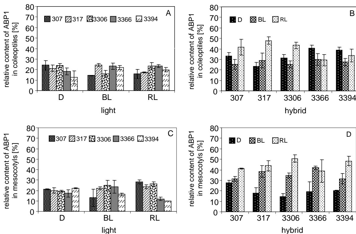
Fig. 6. The amount of ABP1 protein in coleoptiles (A, B) and mesocotyls (C, D) of the 4-day-old maize hybrids grown in D, BL and RL. The amount of protein is compared between the hybrids in certain light condition (A, C), and the effect of light on the ABP1 accumulation is shown separately (B, D). Data are expressed as a percentage of the total area of all signals present on a gel and signal area was determined by ImageJ software. Results represent averages \pm SE obtained from two independent experiments done in duplicates.
